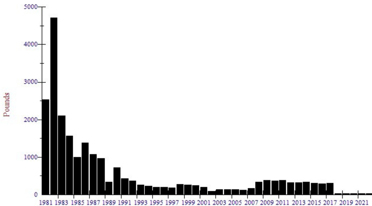
Field's Point Influent Cadmium Loading
