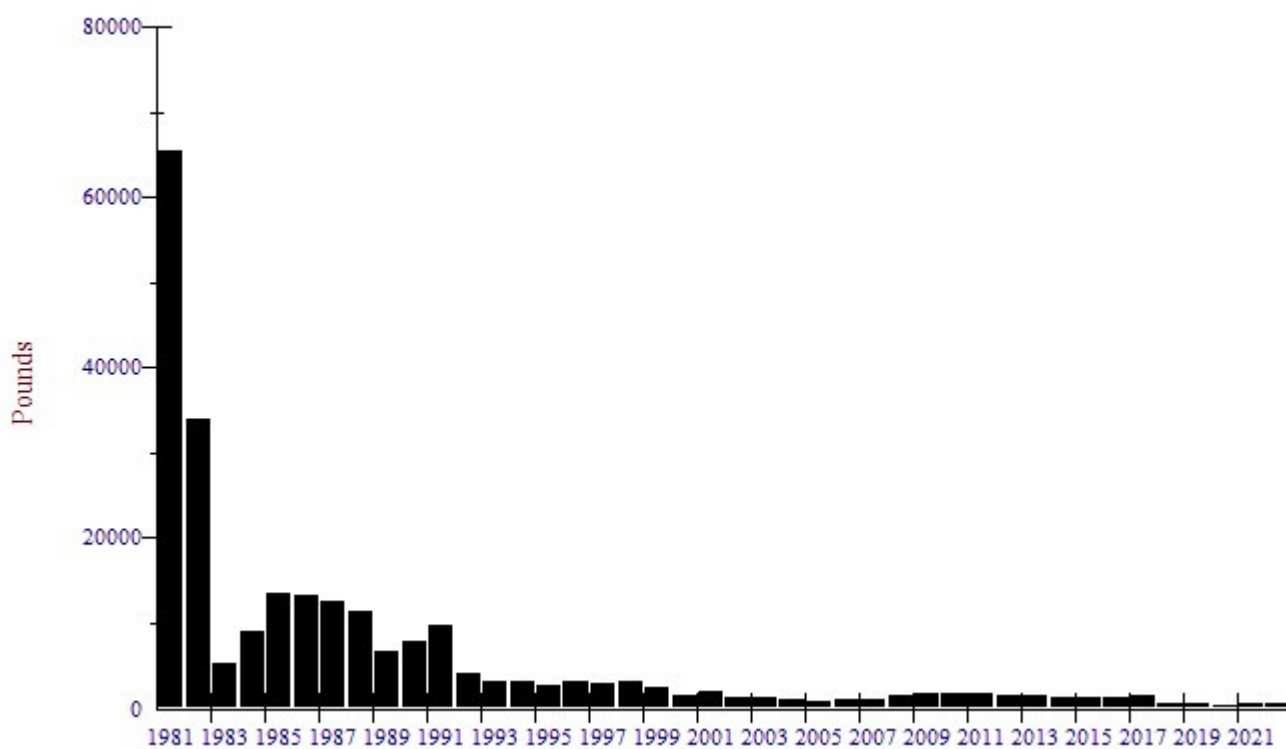
Field's Point Influent Chromium Loading
